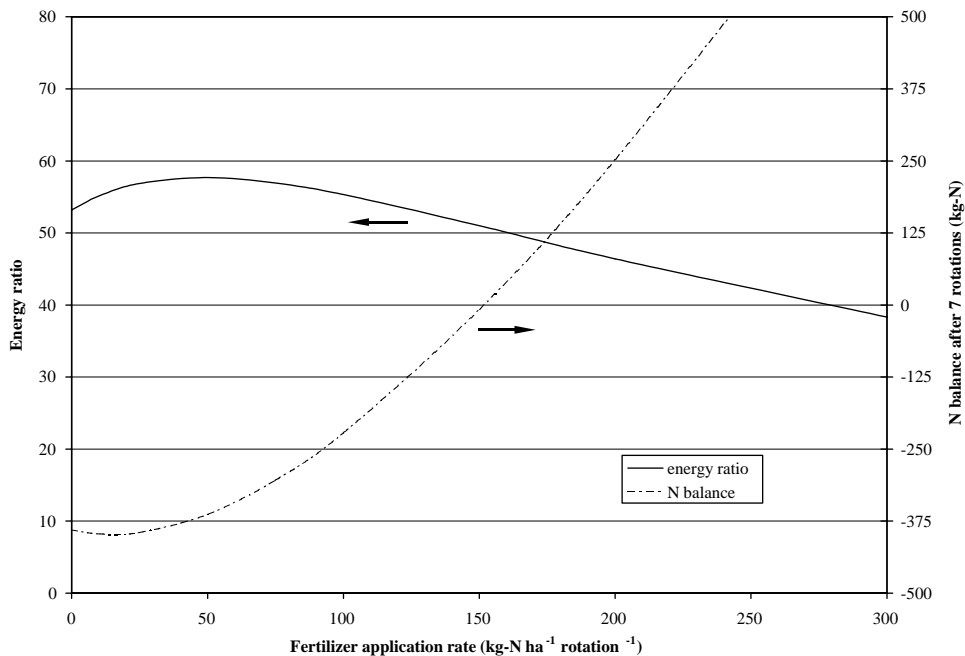
Fig. 4. Net energy ratio (biomass energy at farm gate/ fossil energy consumed) and system nitrogen balance as a function of fertilizer application rate for willow biomass crops grown in New York. Note that the curves are based on limited empirical yield data (see Eq. (3)) and must be considered provisional.
