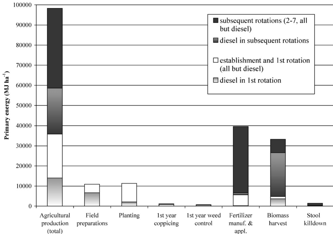
Fig. 2. Primary energy use for major cropping events during the 23 year lifespan of willow biomass crops in New York. “Field preparations” encompasses all of the tilling and weed control activities leading up to planting, including the manufacture of herbicidal inputs. “Planting” includes the nursery production of willow cuttings and the planting operation itself. “Fertilizer manufacturing and application” includes the manufacture and transportation of ammonium sulfate as well as field application of the fertilizer.
