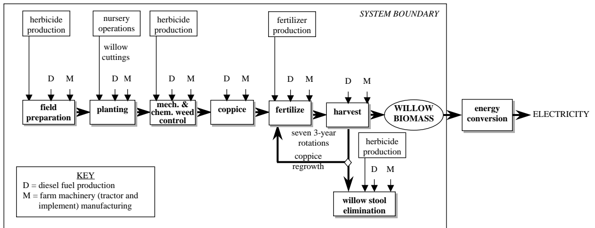
Fig. 1. Schematic of willow biomass cropping system boundary.
