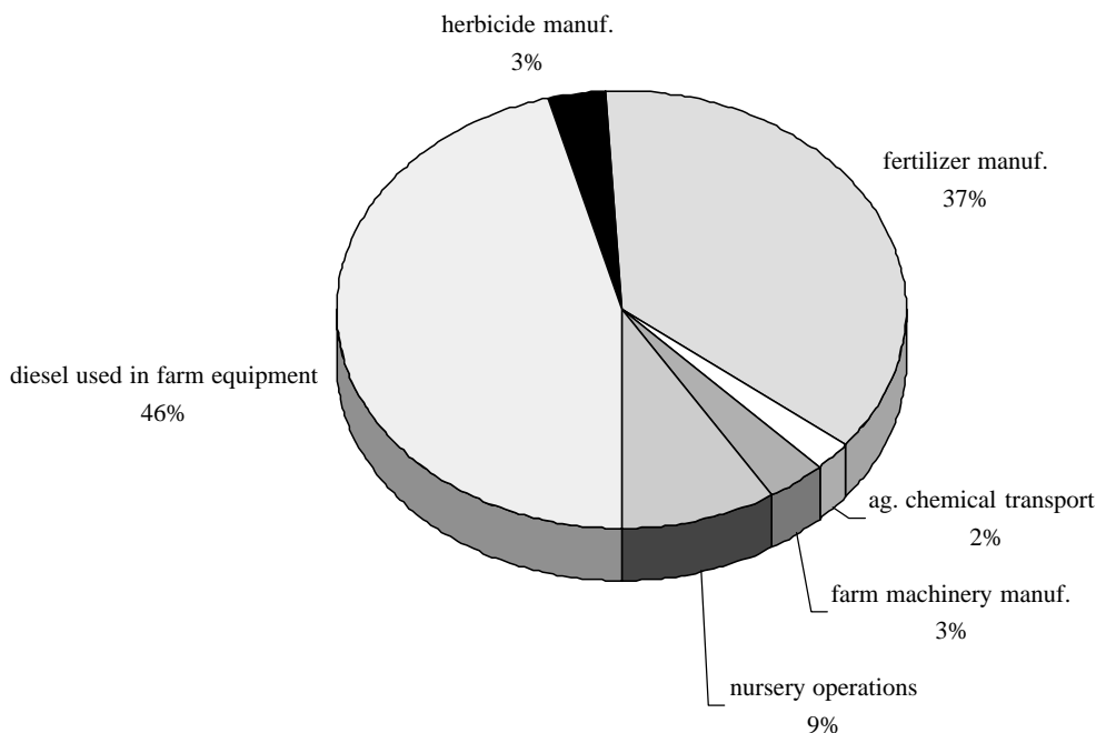
Fig. 3. Breakdown by activity type of primary energy used in producing willow biomass crops.
